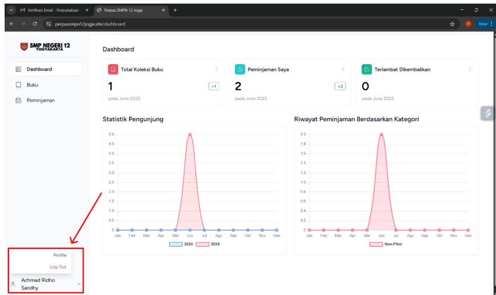
Gambar 42. Menu logout
