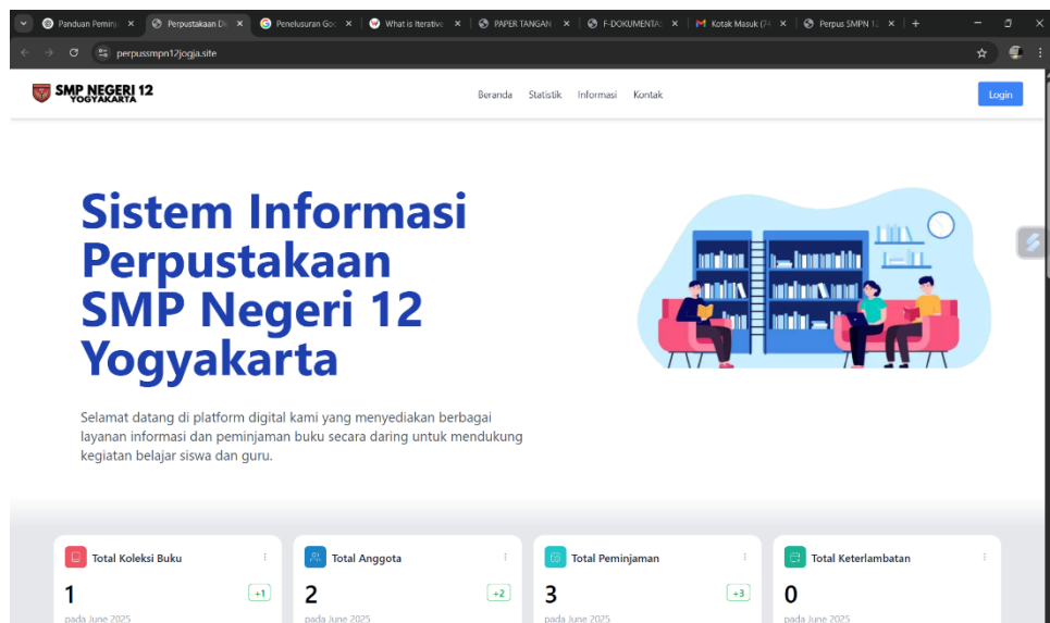
Gambar 2. Welcome Page
