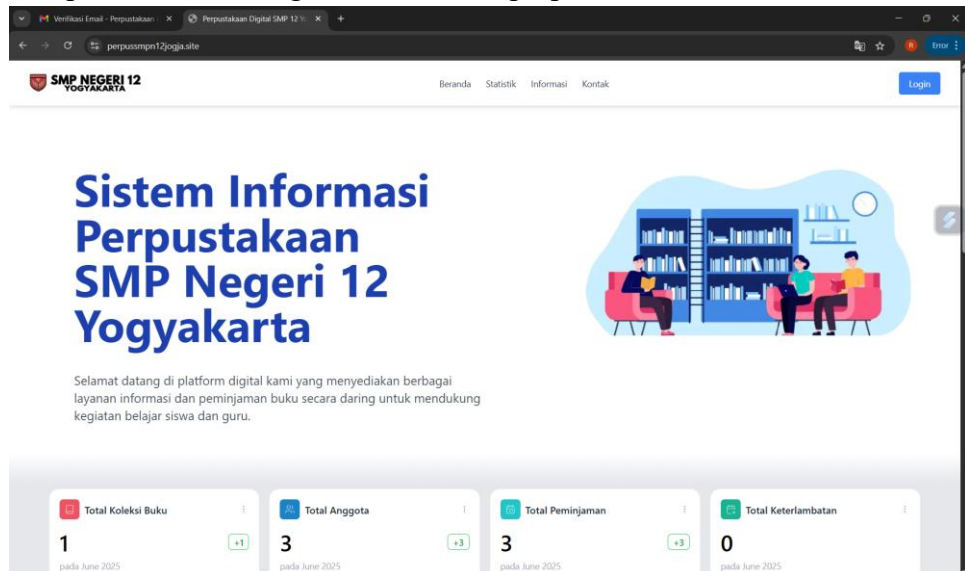
Gambar 43. Welcome page
