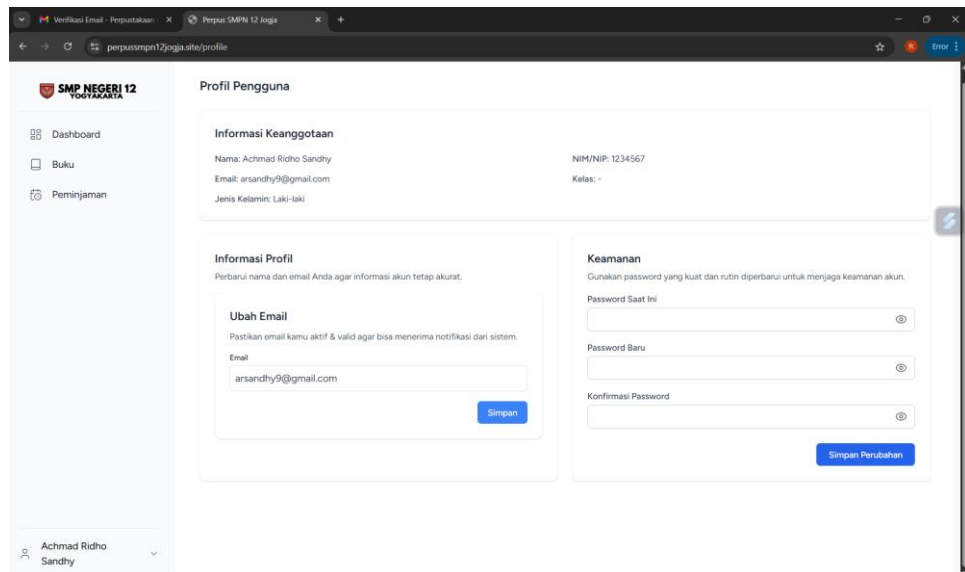
Gambar 40. Profile page
