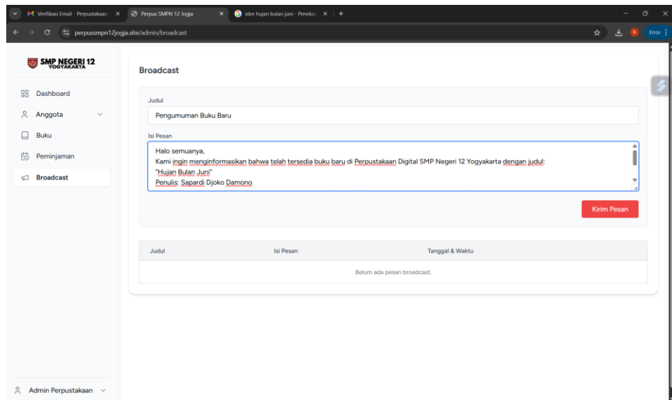
Gambar 23. Broadcast Page
